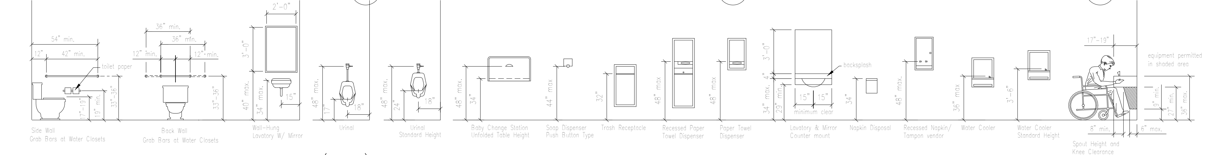
FIXTURE MOUNTING HEIGHTS FOR THE DISABLED ( ADA )
